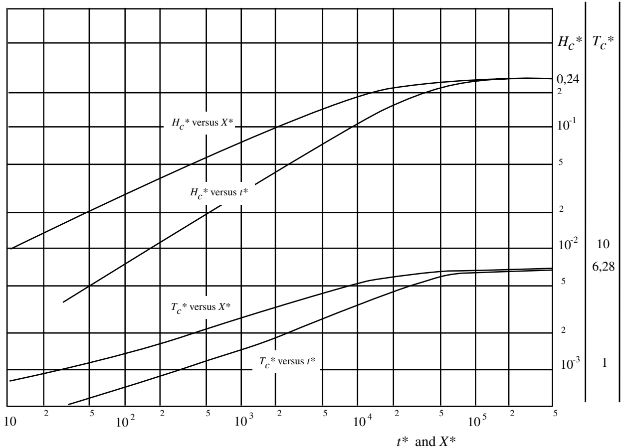
Figure 3.1 — Basic diagram for manual wave forecasting. The curves are drawn for non-dimensional parameters ( H_c^* = gH_c/uv^2 ; T_c^* = gT_c/uv ) (derived from Gröen and Dorrestein, 1976)
